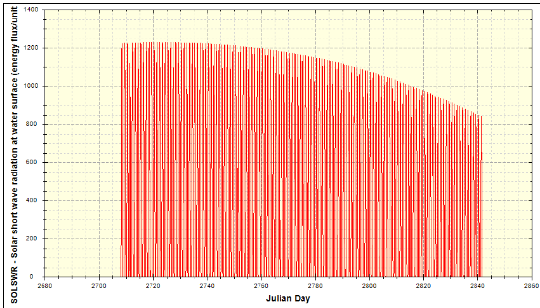
Figure 10: Solar Short wave radiation in Lower Green Bay (W/m 2 )
