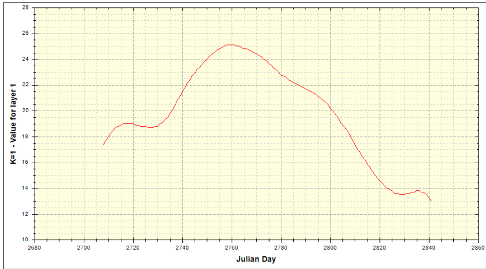
Figure 18: Fox River Temperature (°C); Temperature values were assumed to be uniformly distributed in the vertical direction for all the tributaries
