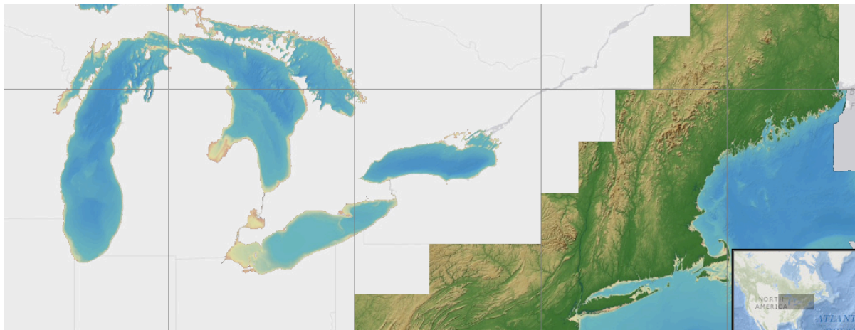
Figure 2: Bathymetry of Lake Michigan(NOAA 2011a)
