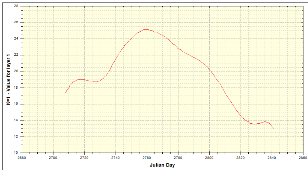
Figure 21: Menominee River Temperature (°C)
